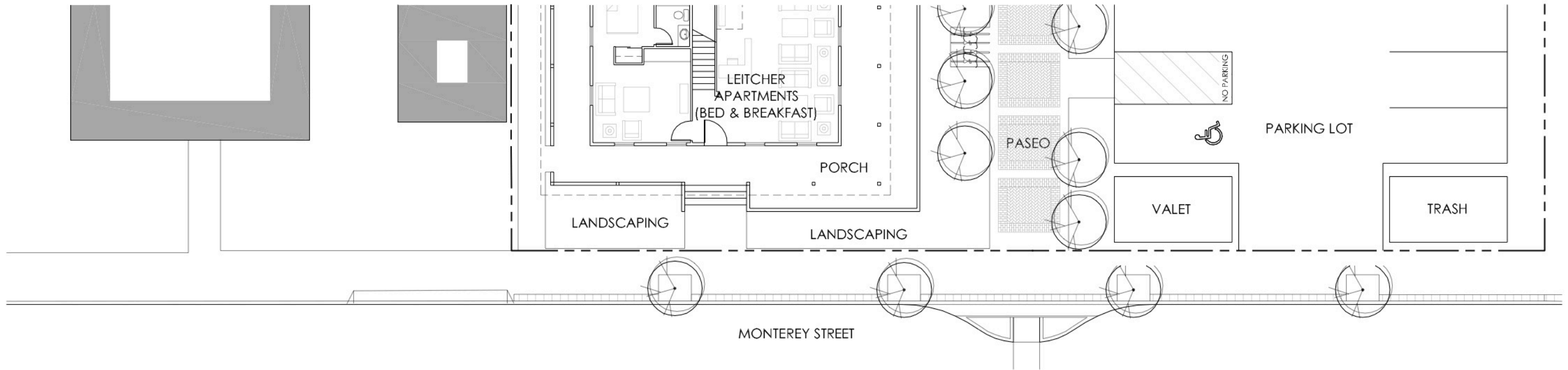
PARTIAL SCHEMATIC SITE PLAN - PHASE 1
